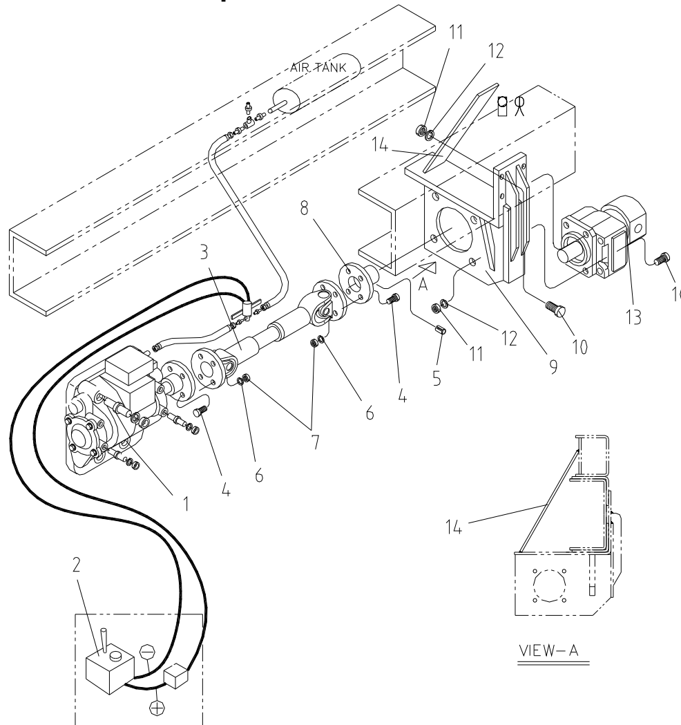
Fig. 8-1 SCS1024LSuper P.T.O &amp; PUMP PART
