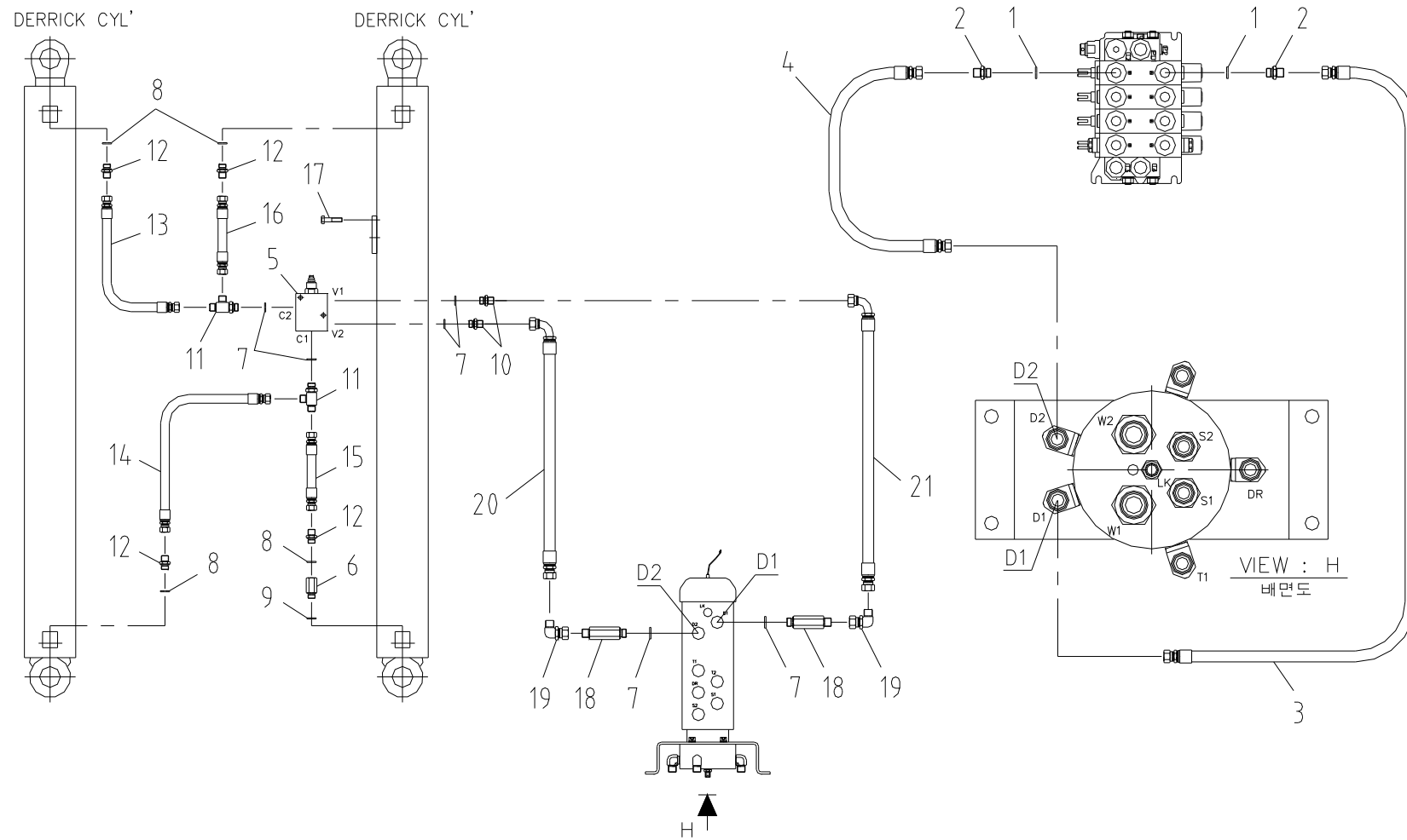
데릭 배관 Fig. 5-2 SCS1024LSuper DERRICK PIPING
