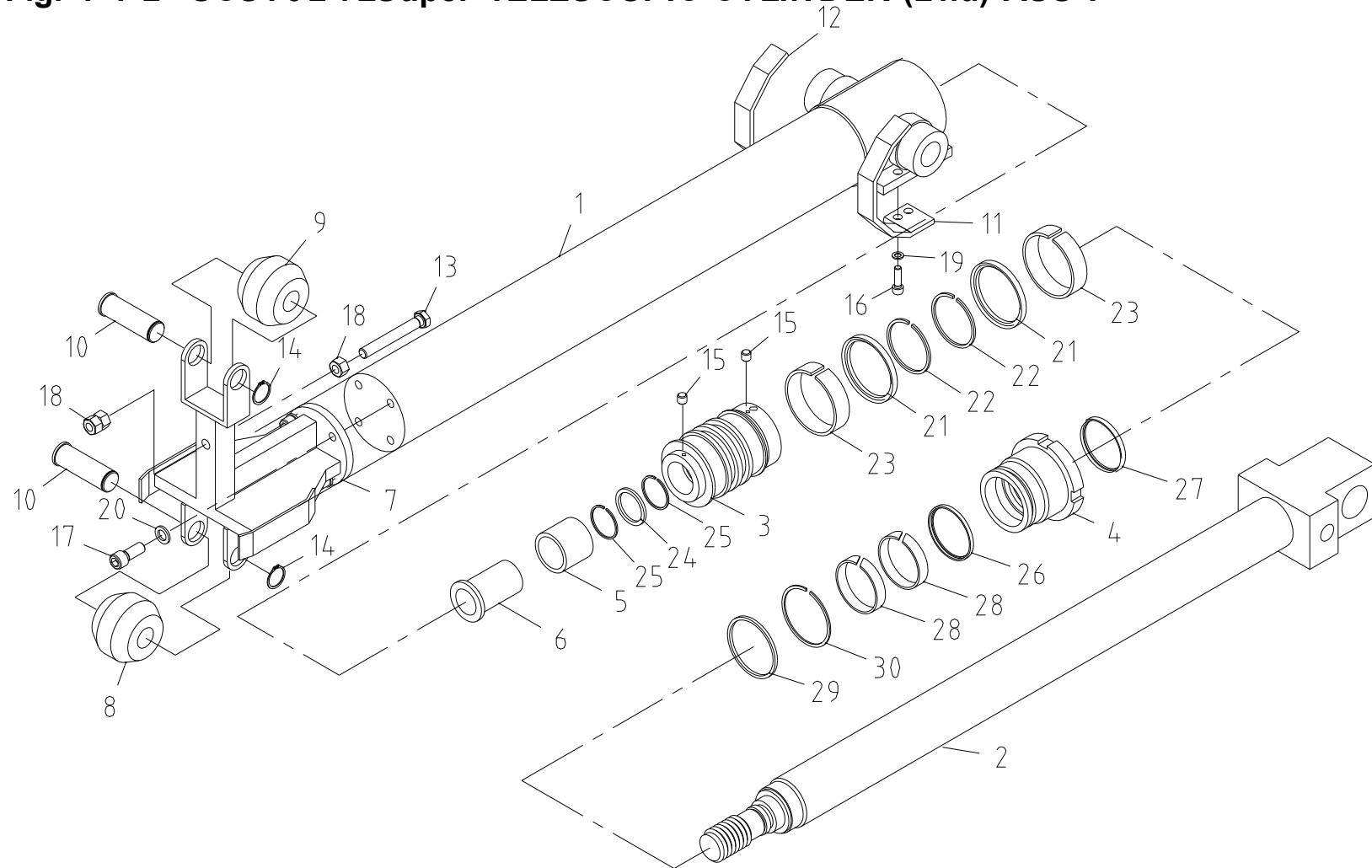
Fig. 1-1-2 SCS1024LSuper TELESCOPIC CYLINDER (2nd) ASS'Y
