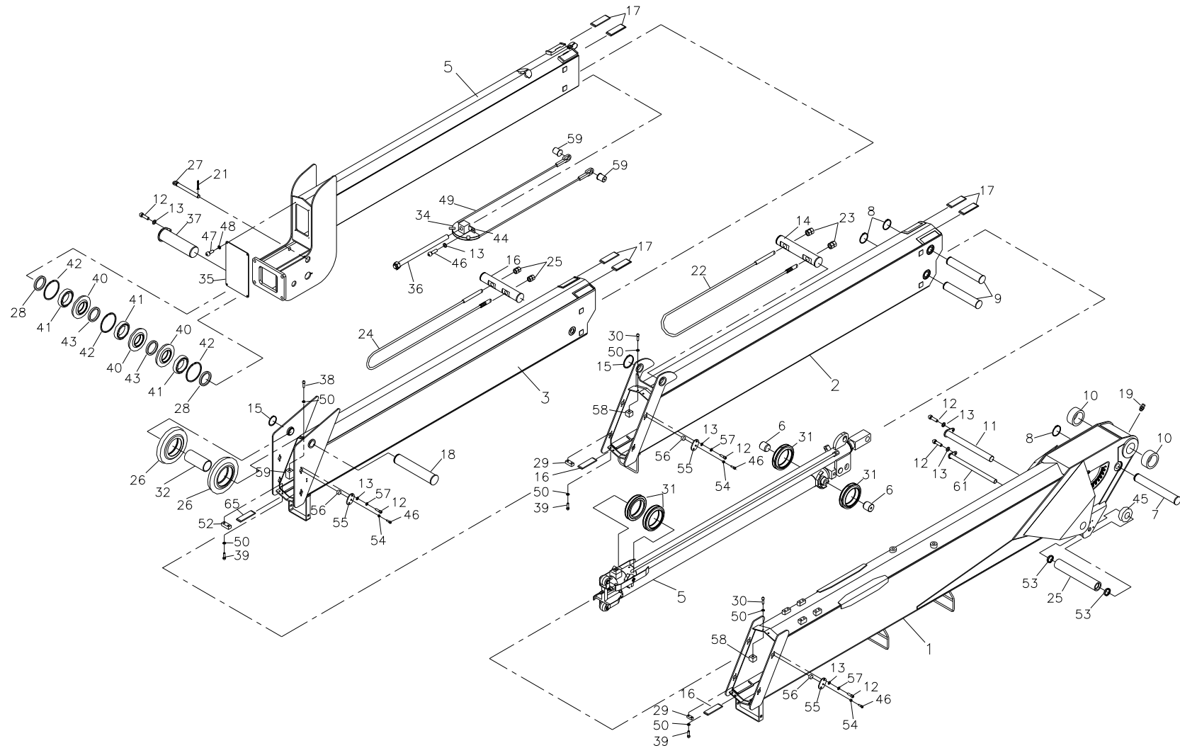
붐 조립체 Fig. 1 SCS1024LSuper BOOM ASS'Y
