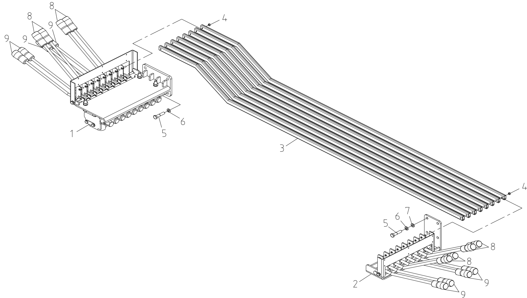
Fig. 3-2 SCS1024LSuper OPERATION ASS'Y (2)
