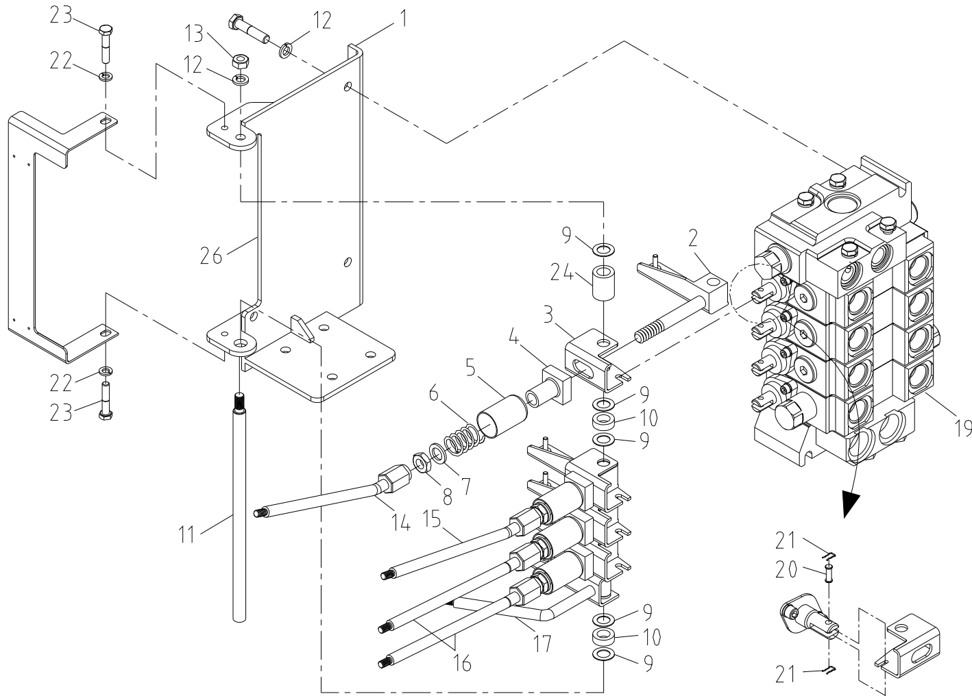
Fig. 3-3-1 SCS1024LSuper VALVE STAND SET
