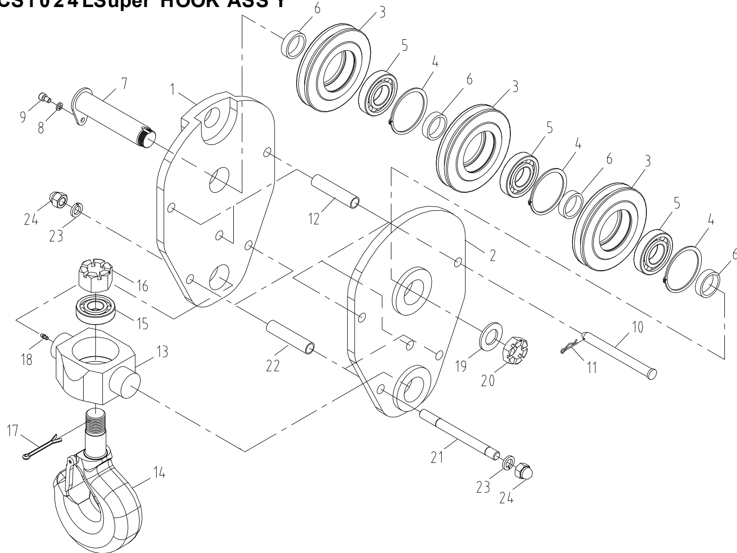
Fig. 7 SCS1024LSuper HOOK ASS'Y
