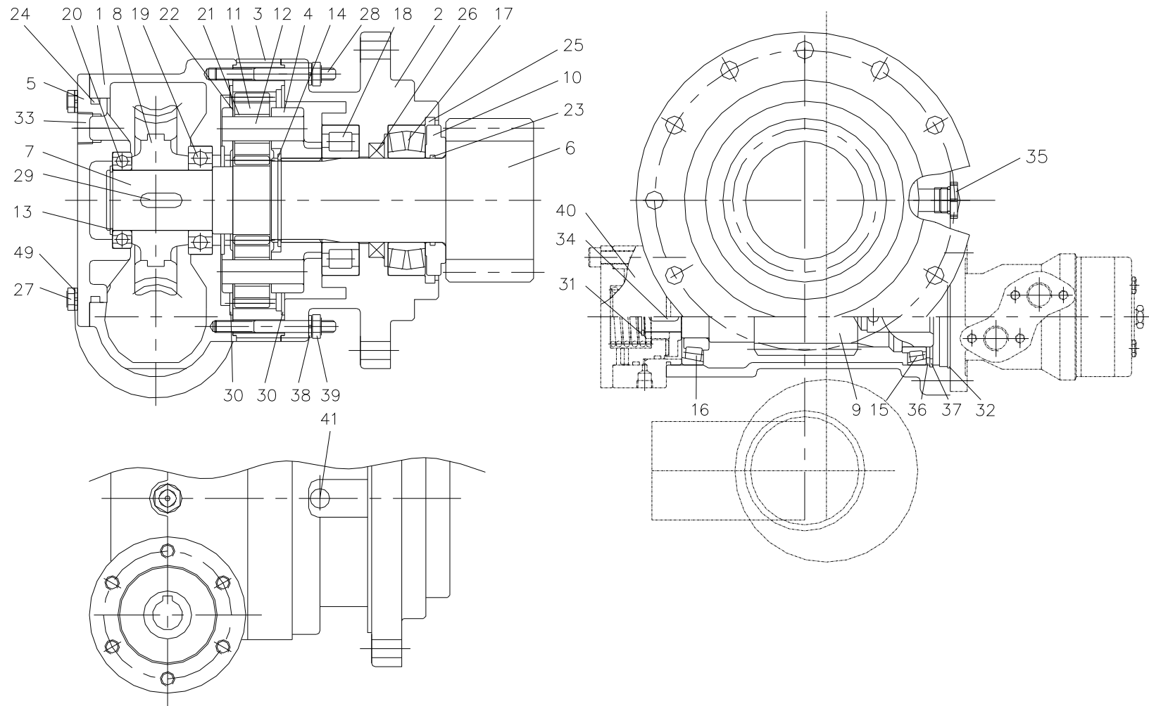
Fig. 2-1 SCS1024LSuper SWING R/ G ASS'Y
