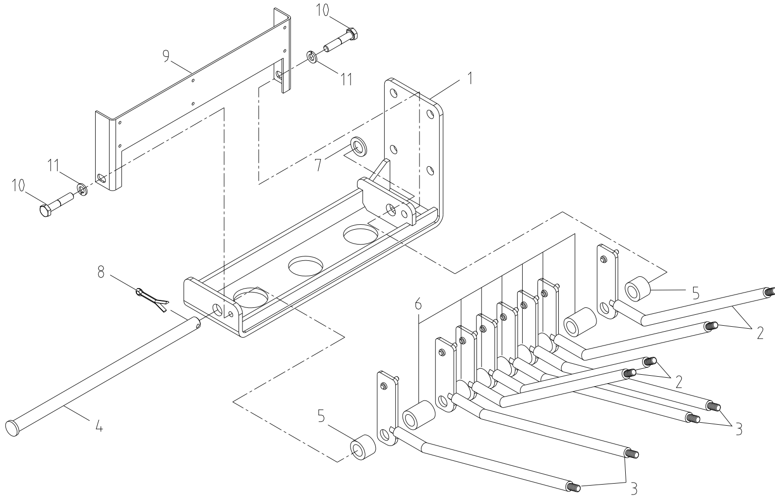
Fig. 3-2-2 SCS1024LSuper LEVER STAND SET
