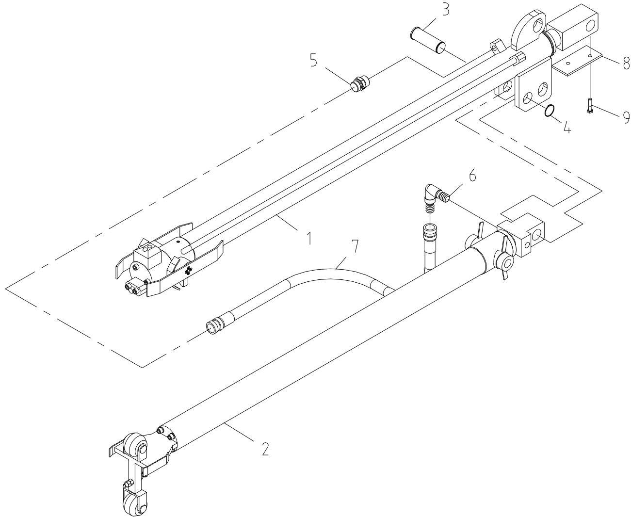
Fig. 1-1 SCS1024LSuper TELESCOPIC CYLINDER ASS'Y
